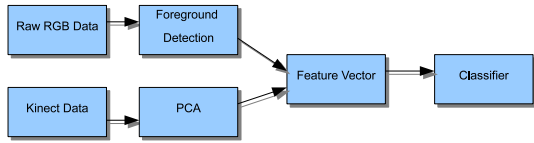
Figure 6: Overview of data fusion classification method A.
