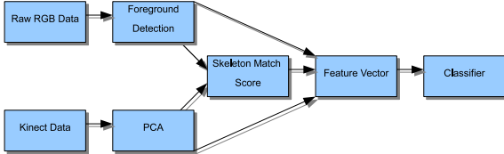
Figure 7: Overview of data fusion classification method B.
