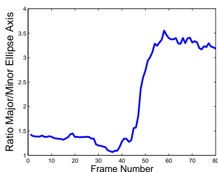
Figure 5: The ellipse major/minor axis ratio during a fall. Fall occurs between frames 40 and 60 (frame rate is 15 fps).
